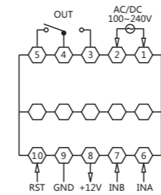
CA4 wire connection
