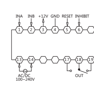
CA7 wire connection
