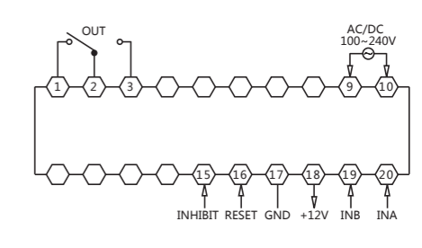
CA8 wire connection
